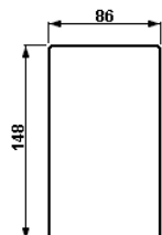
Flange opening for GHG 412 82
